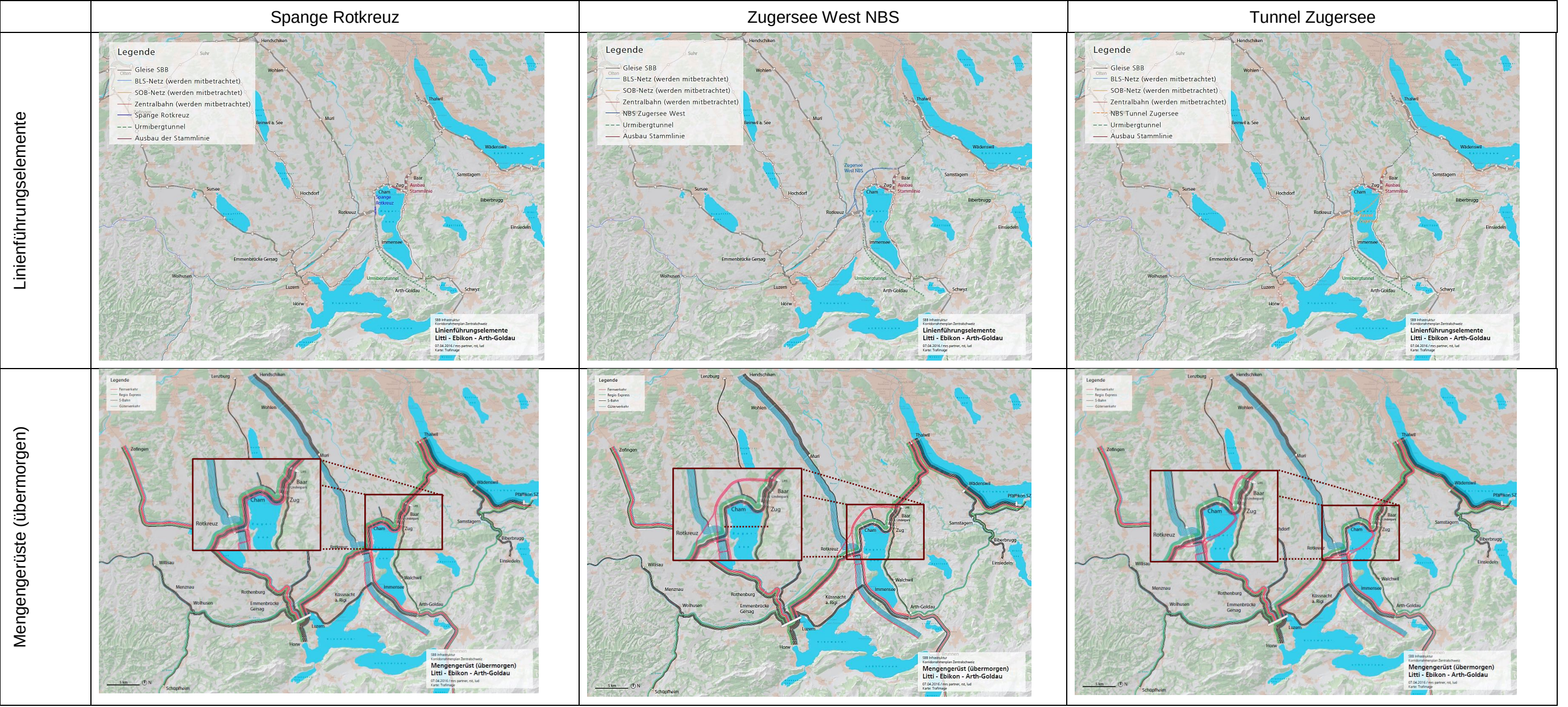
Abb. 44: Variantenfächer Litti–Ebikon/Arth-Goldau
